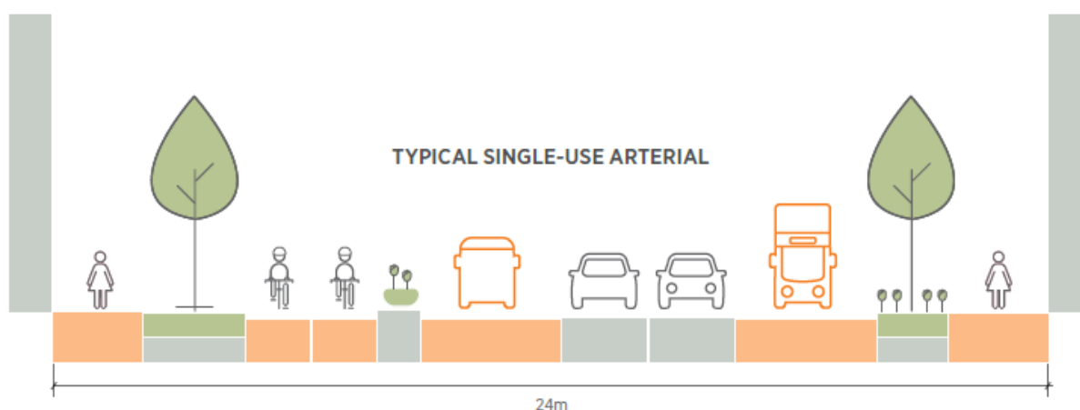
Figure 3-14: Cross-section of a future Auckland arterial road
