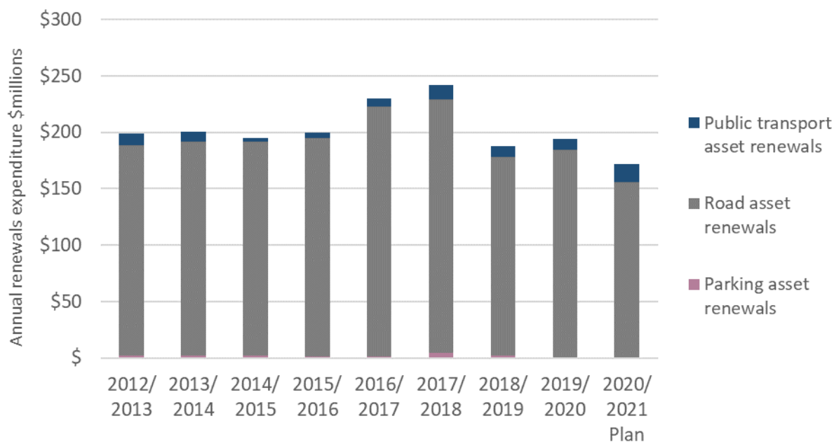
Figure 3-5: Past (actual) and current (planned) costs to renew road and public transport assets
