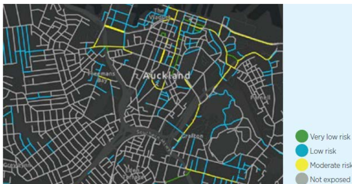
Figure 7-4: Sealed roads – evidence of criticality and resilience
