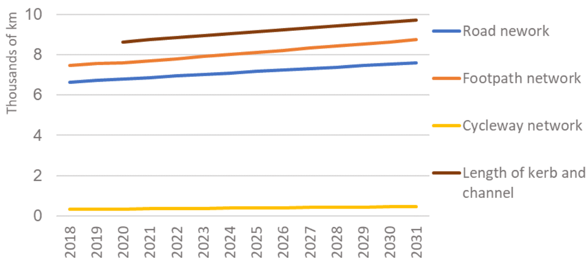
Figure 3-20: Actual and forecast growth in road assets
