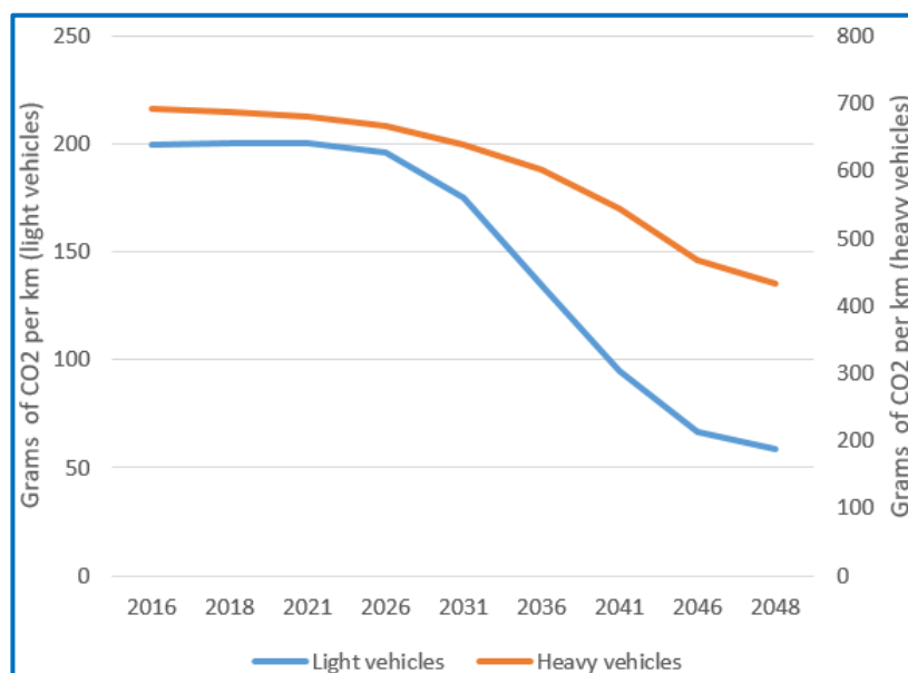
Figure 46 - Forecast reduction in NZ vehicle fleet CO 2 emissions 78
