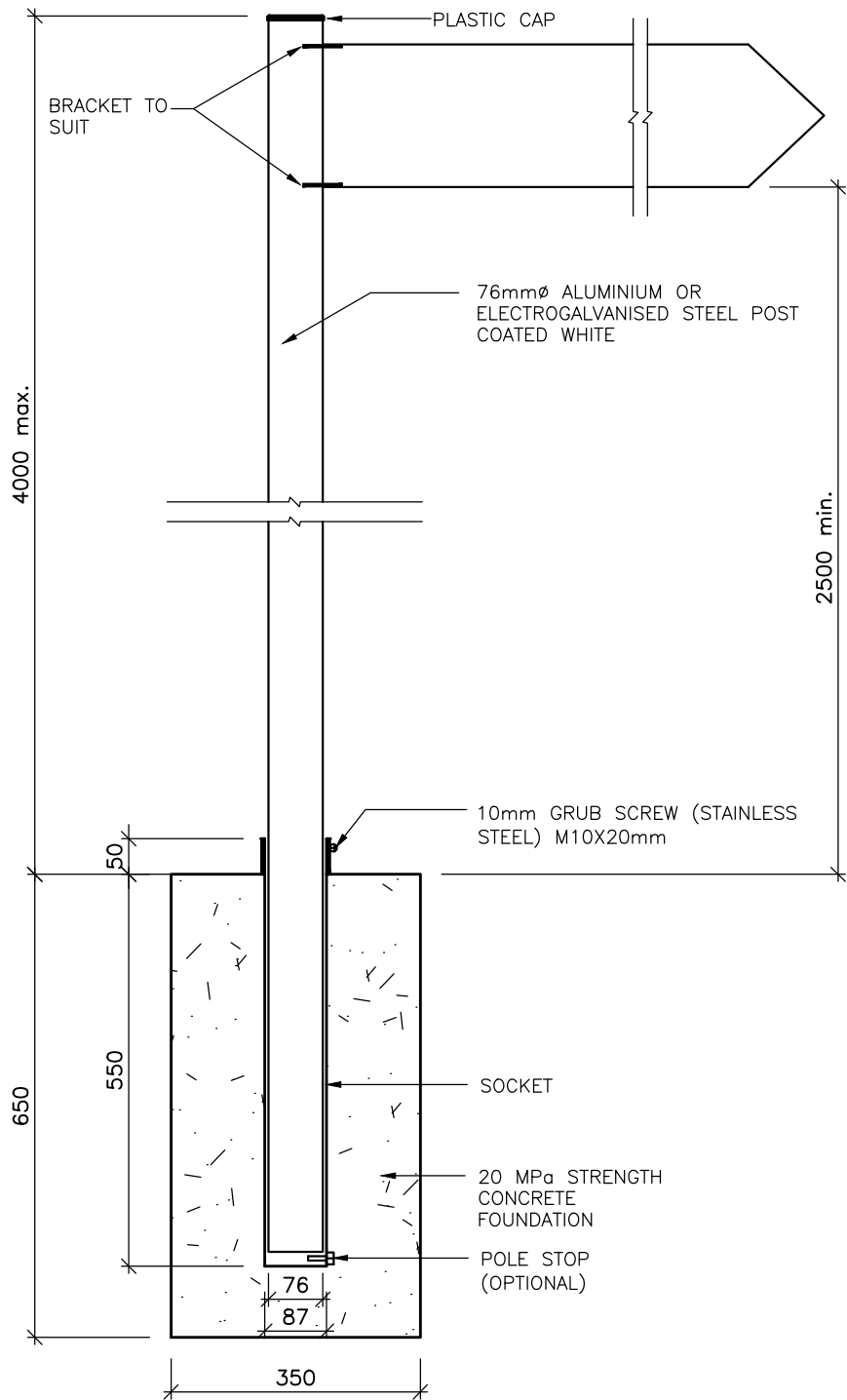
TYPICAL DETAIL SCALE 1:10
