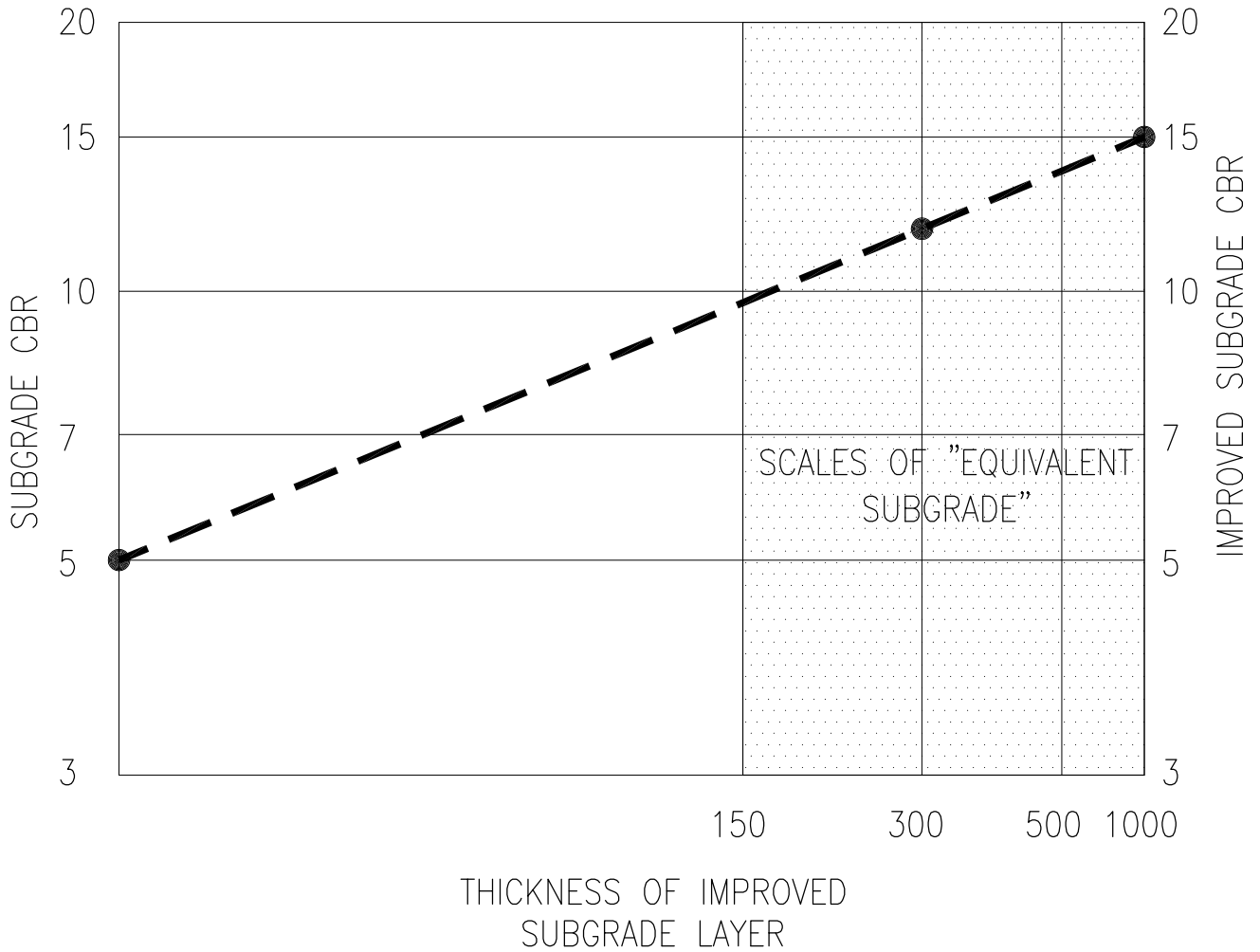
NOMOGRAPH FOR DETERMINING THE EFFECT OF SUBGRADE IMPROVEMENT LAYERS
